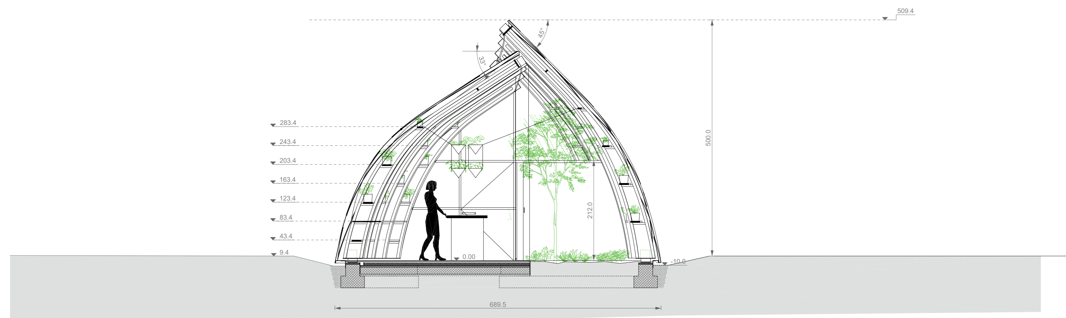
SECTION A
